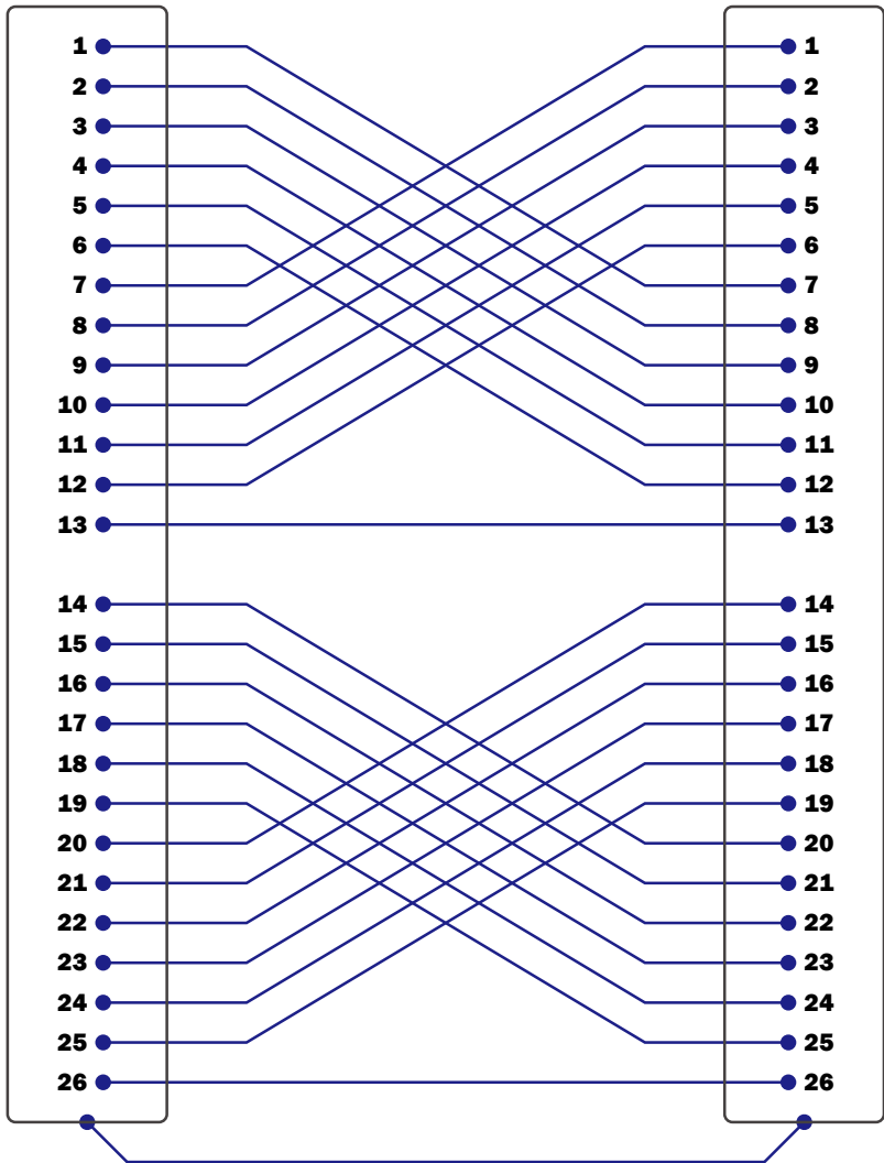
26-pin Hirose DXM series connectors
